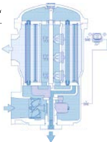
BOLLFILTER Automa Type 6.46
