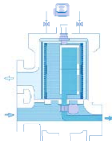
BOLLFILTER Type 6.21
