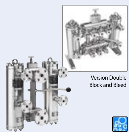
BOLLFILTER Duplex Type BFD-C
